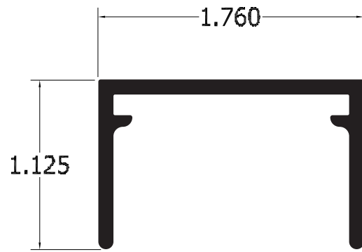
SERIES 2 FRAMELESS BODY PART#1125
